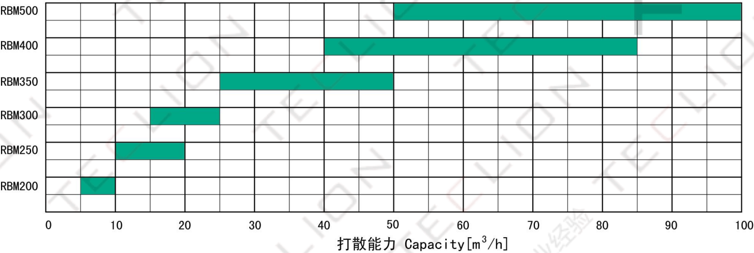
处理能力基于含湿量不超过20%粉块 Capacity based on the water content of not more than 20% powder chunk
